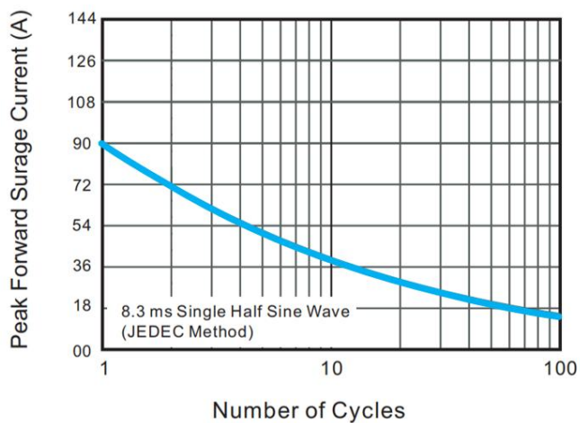
Figure 3. Forward Surge Current Derating Curve
